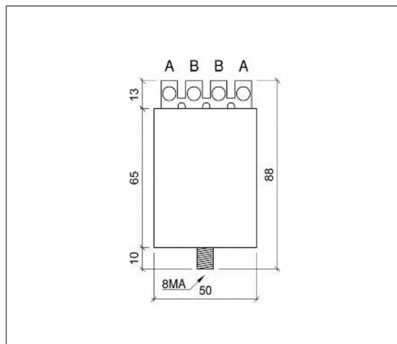
Ignitor DI19 Dimensions
