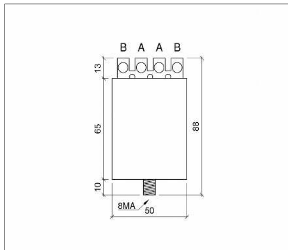
Ignitor DI17 Dimensions
